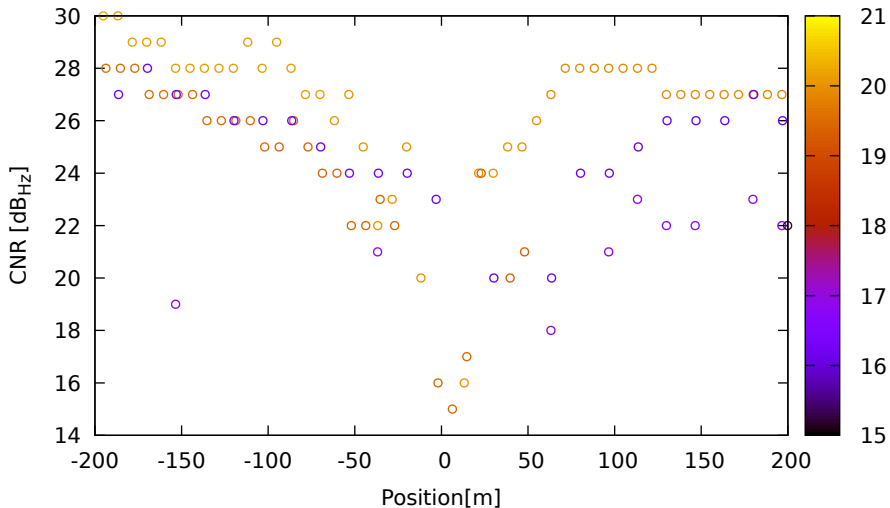
CNR vs position for C11 (B1) on HuaweiP40 - DOY 262 jam. 1
