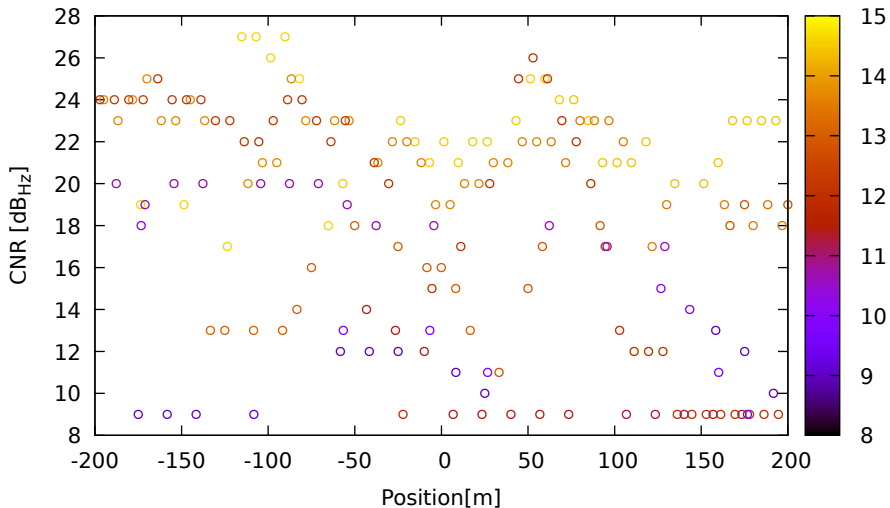
CNR vs position for C11 (B1) on HuaweiP40 - DOY 262 jam. 2
