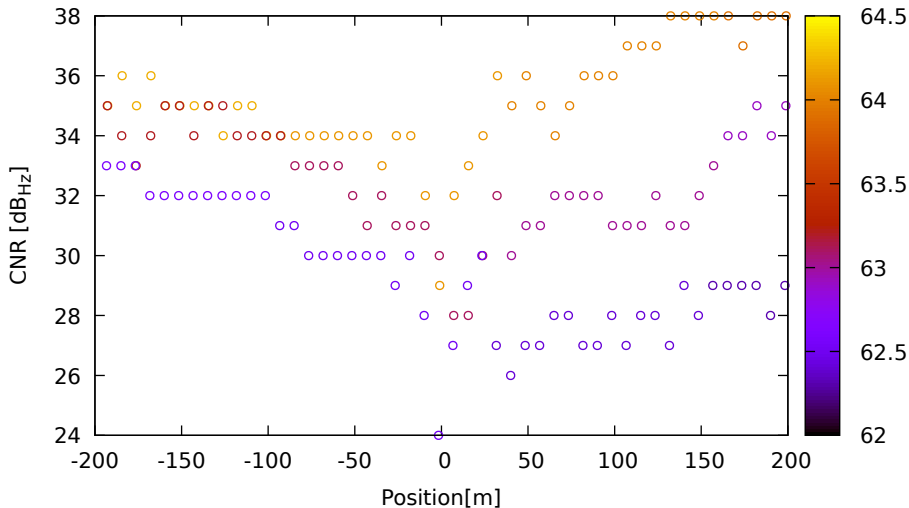
CNR vs position for C14 (B1) on HuaweiP40 - DOY 262 jam. 3
