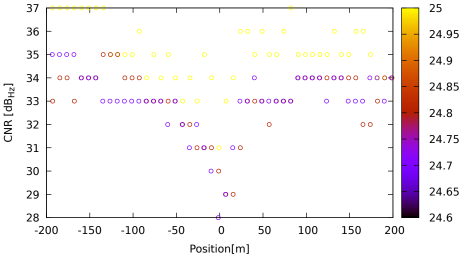
CNR vs position for C16 (B1) on HuaweiP40 - DOY 262 jam. 3
