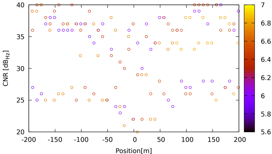
CNR vs position for C26 (B1) on HuaweiP40 - DOY 262 jam. 3
