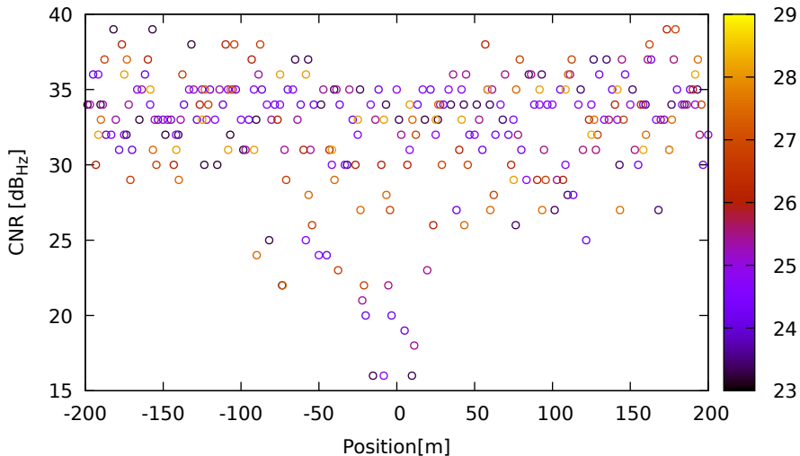
CNR vs position for C27 (B1) on HuaweiP40 - DOY 262 jam. 2
