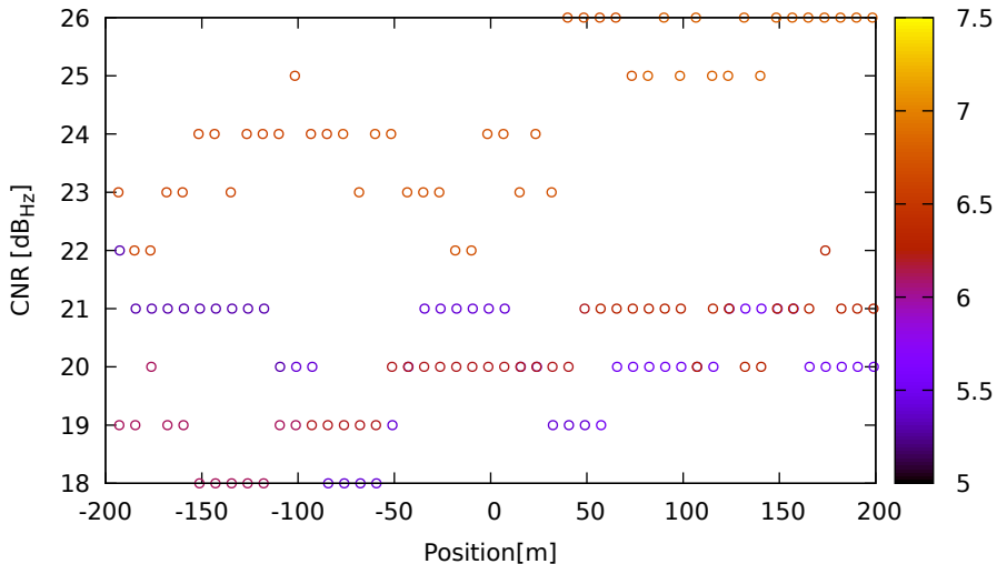
CNR vs position for E03 (E1) on HuaweiP40 - DOY 262 jam. 3
