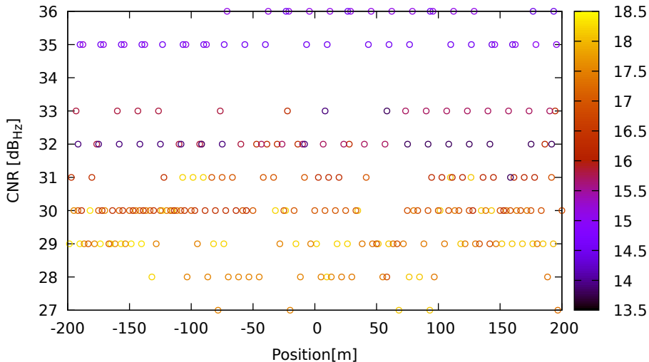
CNR vs position for E04 (E1) on HuaweiP40 - DOY 262 jam. 2
