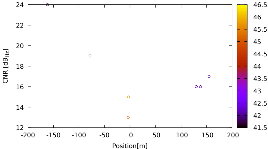
CNR vs position for E05 (E5a) on HuaweiP40 - DOY 262 jam. 1
