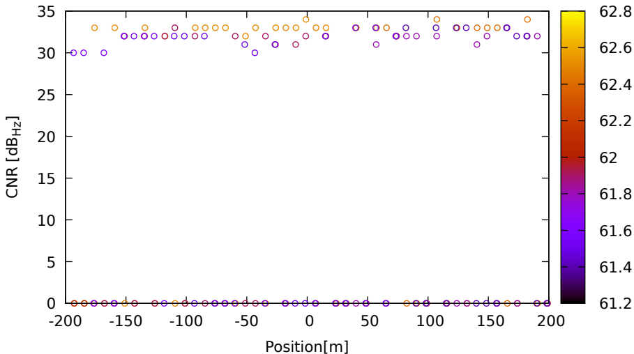
CNR vs position for E09 (E1) on HuaweiP40 - DOY 262 jam. 3
