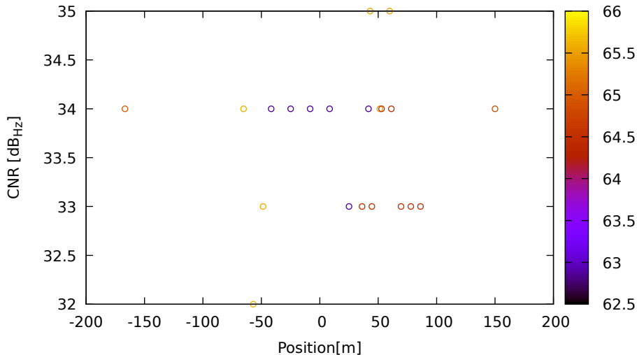
CNR vs position for E09 (E5a) on HuaweiP40 - DOY 262 jam. 2
