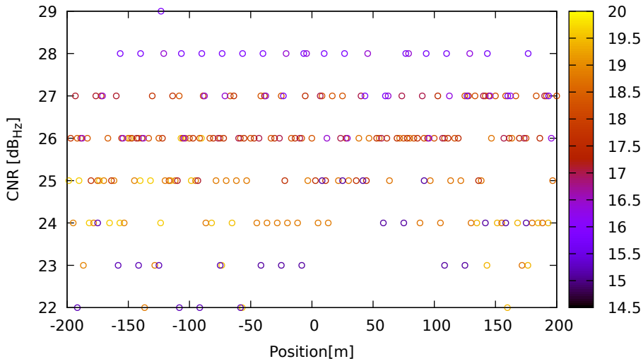
CNR vs position for E11 (E1) on HuaweiP40 - DOY 262 jam. 2
