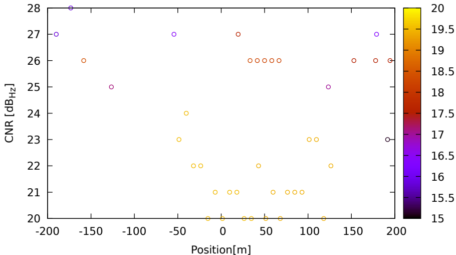
CNR vs position for E11 (E5a) on HuaweiP40 - DOY 262 jam. 2
