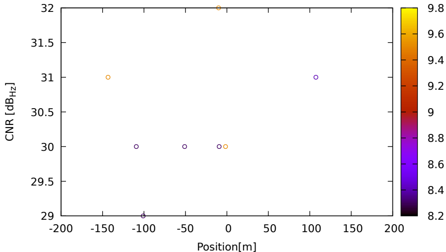
CNR vs position for E15 (E5a) on HuaweiP40 - DOY 262 jam. 3
