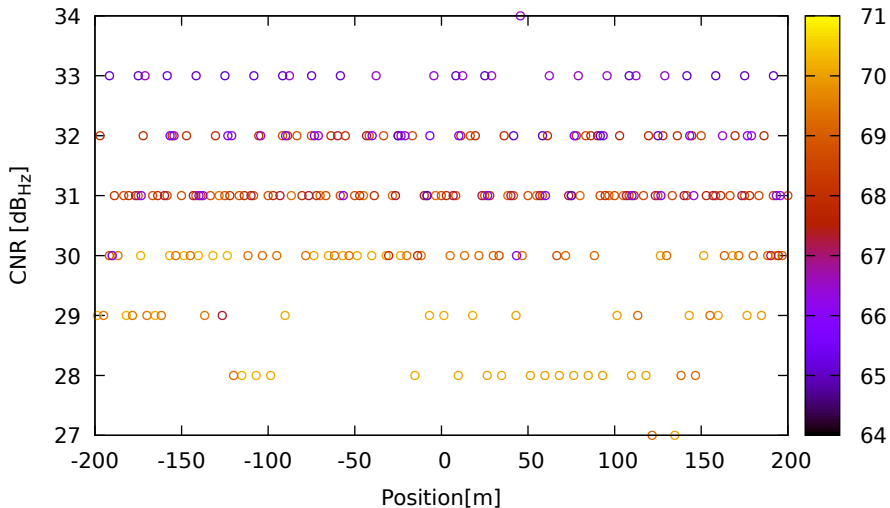
CNR vs position for E36 (E1) on HuaweiP40 - DOY 262 jam. 2
