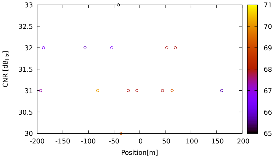
CNR vs position for E36 (E5a) on HuaweiP40 - DOY 262 jam. 2
