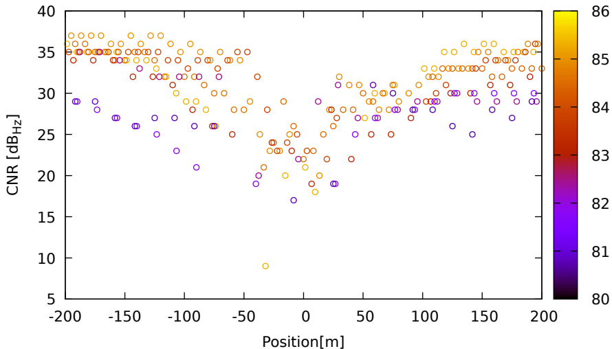
CNR vs position for G01 (L1) on HuaweiP40 - DOY 262 jam. 2
