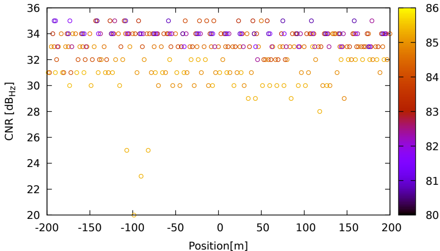
CNR vs position for G01 (L5) on HuaweiP40 - DOY 262 jam. 2
