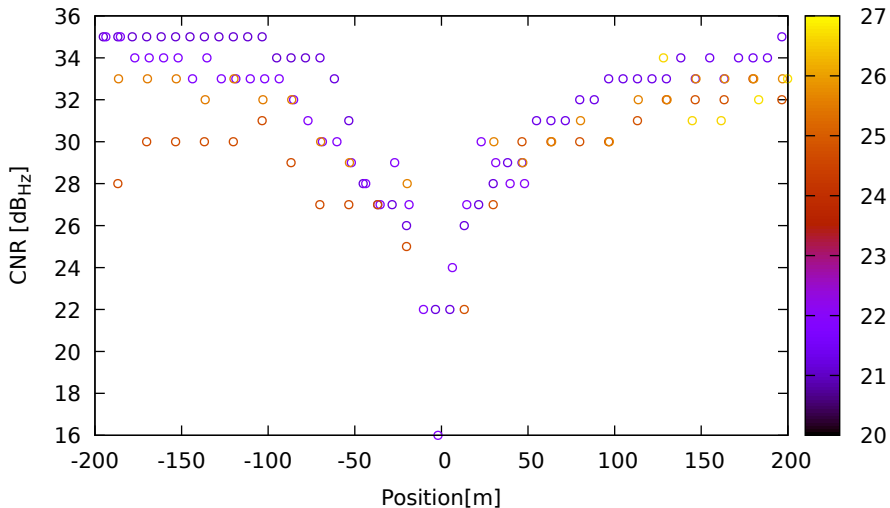
CNR vs position for G04 (L1) on HuaweiP40 - DOY 262 jam. 1
