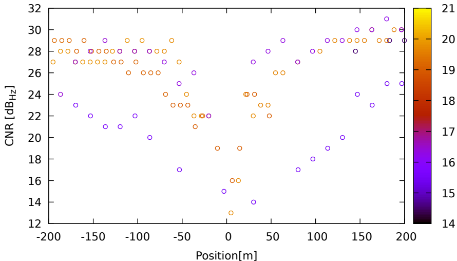
CNR vs position for G08 (L1) on HuaweiP40 - DOY 262 jam. 1
