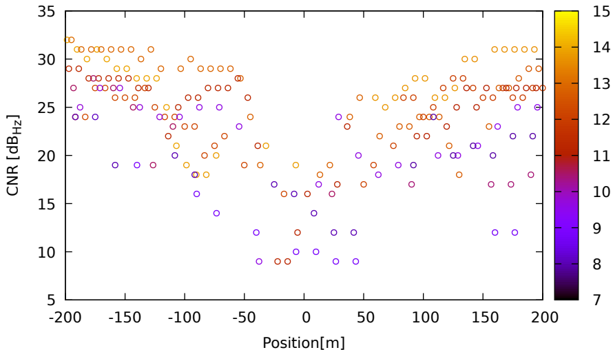
CNR vs position for G08 (L1) on HuaweiP40 - DOY 262 jam. 2
