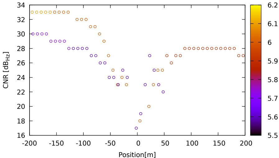
CNR vs position for G14 (L1) on HuaweiP40 - DOY 262 jam. 1
