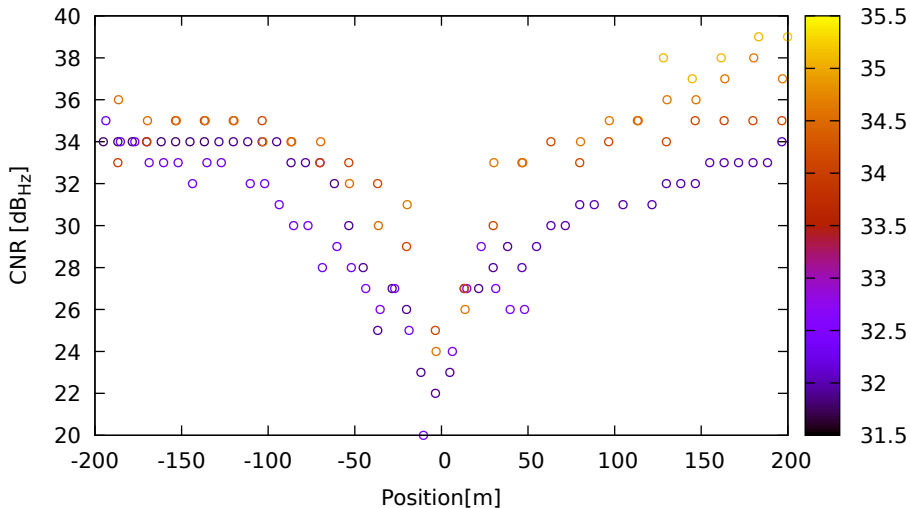
CNR vs position for G17 (L1) on HuaweiP40 - DOY 262 jam. 1
