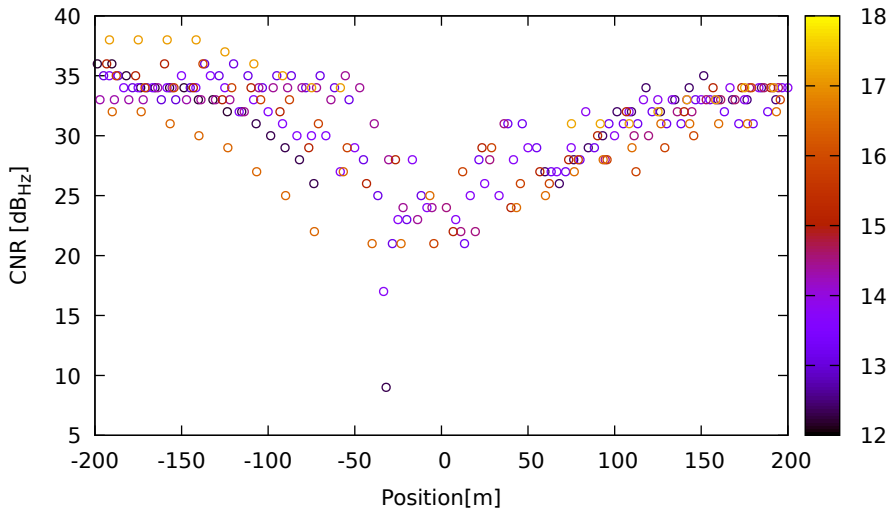
CNR vs position for G19 (L1) on HuaweiP40 - DOY 262 jam. 2
