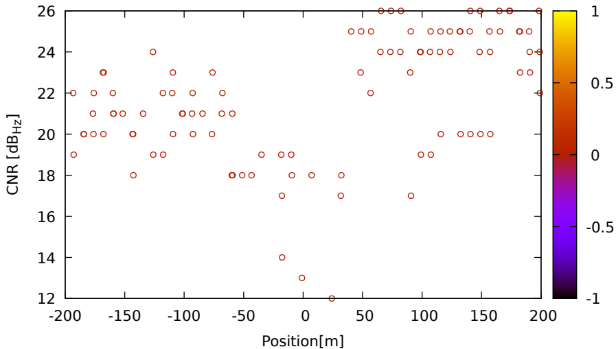
CNR vs position for G28 (L1) on HuaweiP40 - DOY 262 jam. 3
