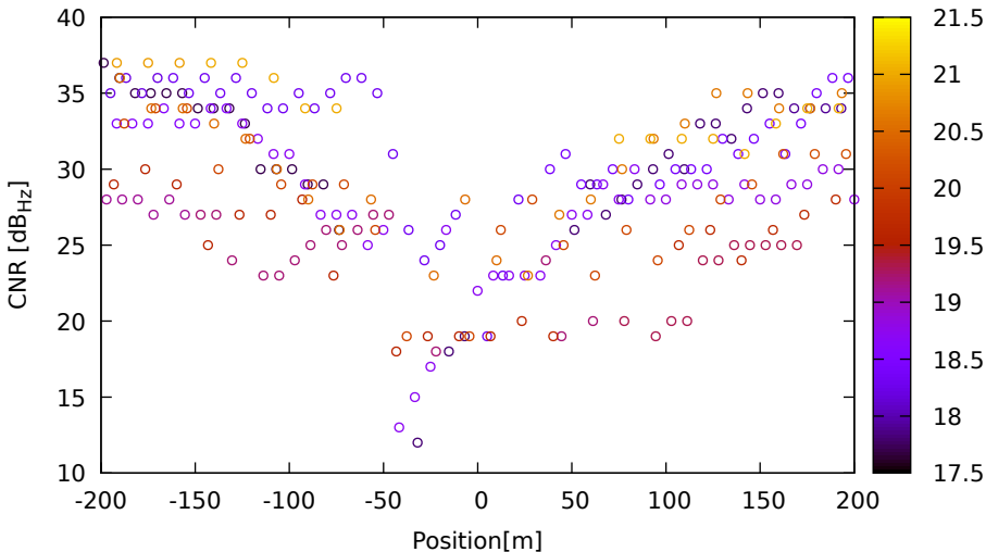
CNR vs position for G31 (L1) on HuaweiP40 - DOY 262 jam. 2
