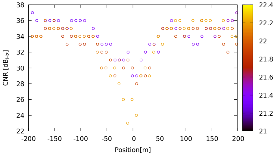
CNR vs position for G31 (L1) on HuaweiP40 - DOY 262 jam. 3
