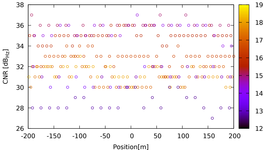
CNR vs position for G32 (L5) on HuaweiP40 - DOY 262 jam. 2
