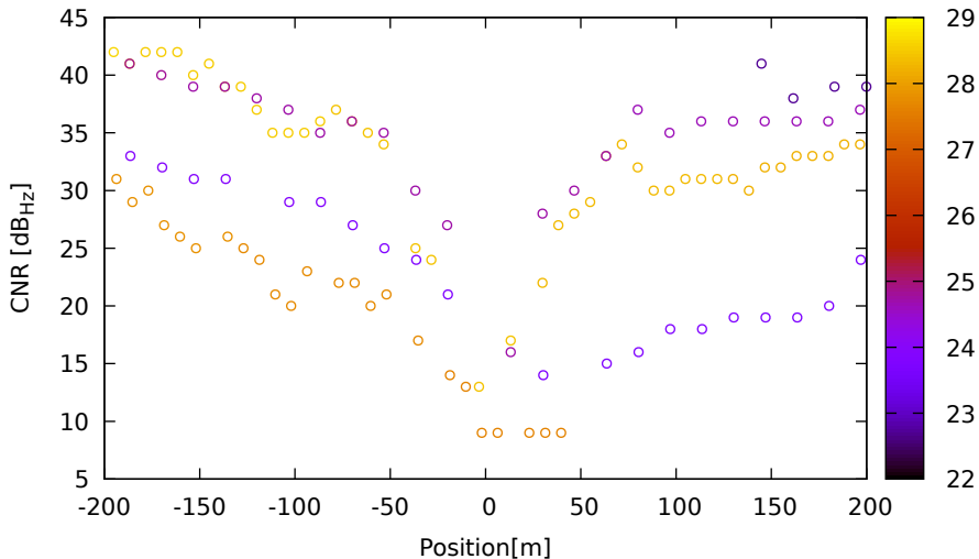
CNR vs position for R07 (G1) on HuaweiP40 - DOY 262 jam. 1
