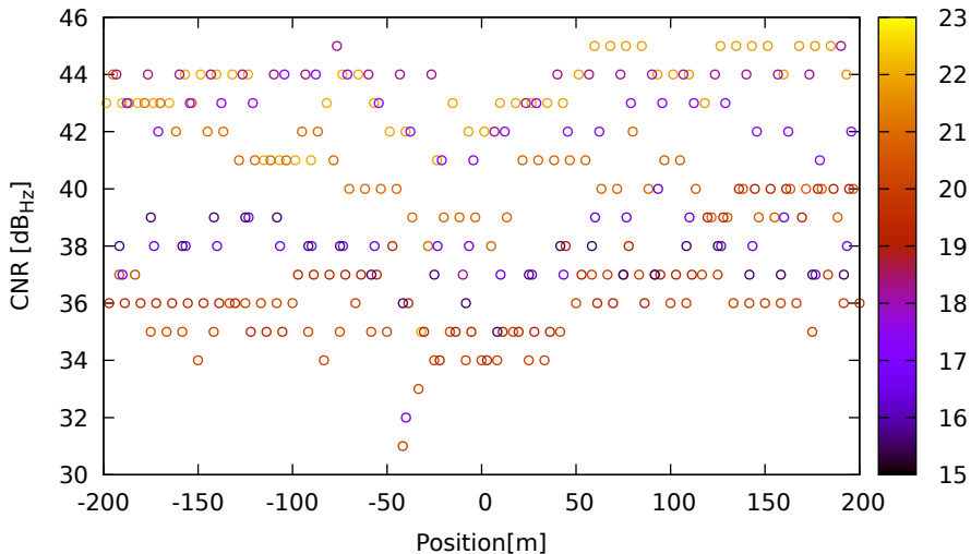
CNR vs position for R07 (G1) on HuaweiP40 - DOY 262 jam. 2
