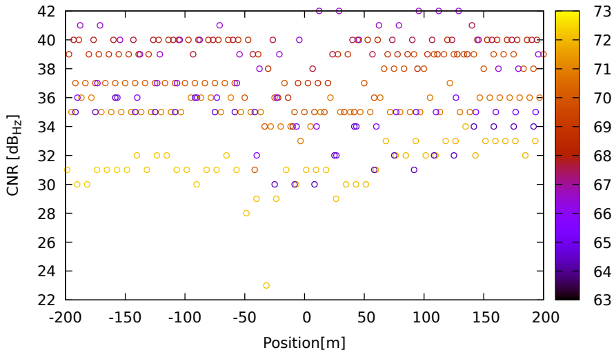
CNR vs position for R08 (G1) on HuaweiP40 - DOY 262 jam. 2
