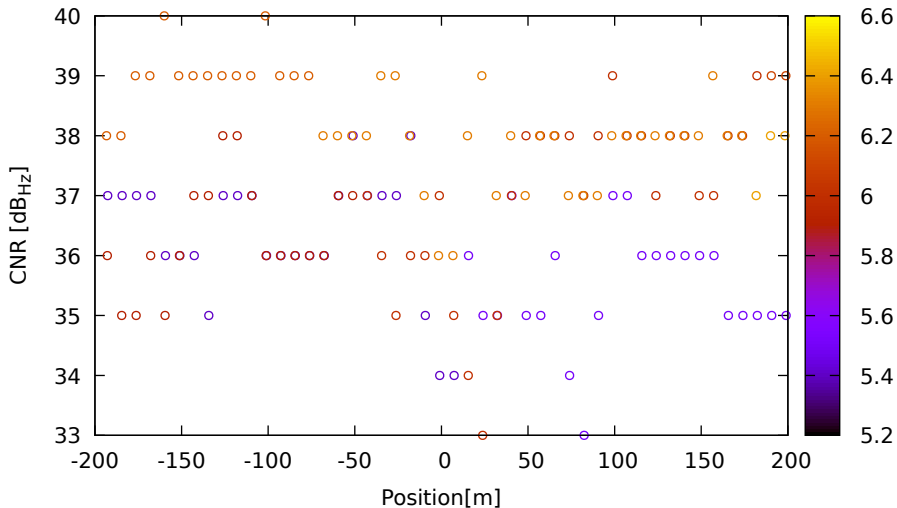
CNR vs position for R09 (G1) on HuaweiP40 - DOY 262 jam. 3
