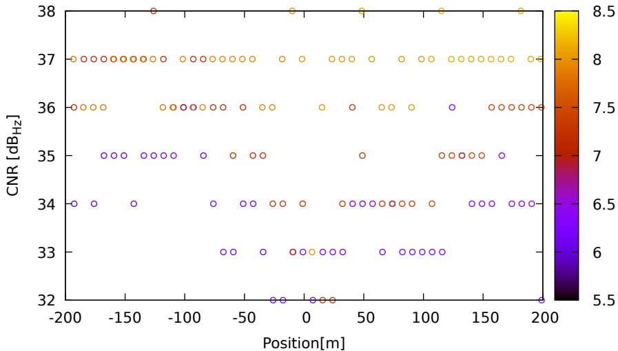
CNR vs position for R17 (G1) on HuaweiP40 - DOY 262 jam. 3
