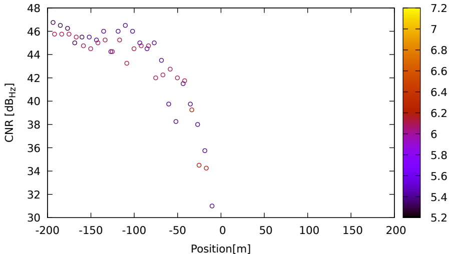
CNR vs position for E03 (E1) on LeicaGS15 - DOY 262 jam. 3
