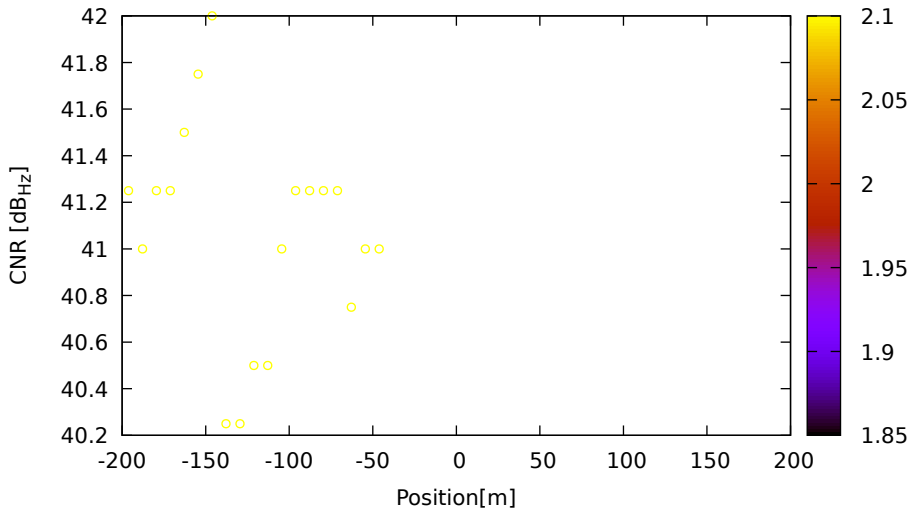
CNR vs position for E03 (E5a) on LeicaGS15 - DOY 262 jam. 2
