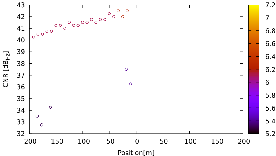
CNR vs position for E03 (E5a) on LeicaGS15 - DOY 262 jam. 3
