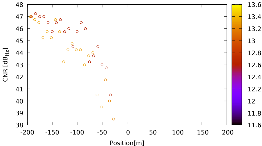
CNR vs position for E04 (E1) on LeicaGS15 - DOY 262 jam. 3
