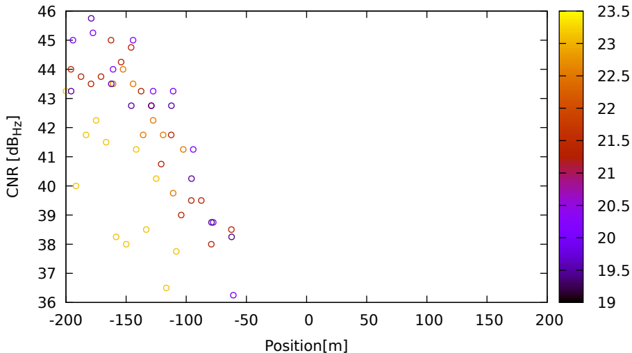
CNR vs position for E04 (E5b) on LeicaGS15 - DOY 262 jam. 1
