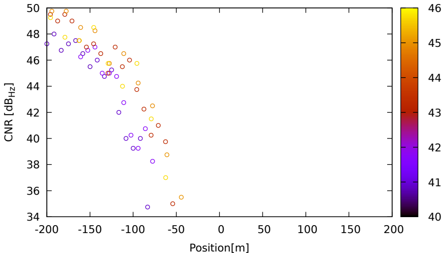
CNR vs position for E05 (E1) on LeicaGS15 - DOY 262 jam. 1
