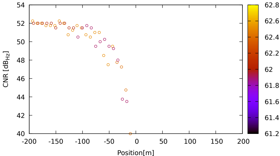
CNR vs position for E09 (E1) on LeicaGS15 - DOY 262 jam. 3
