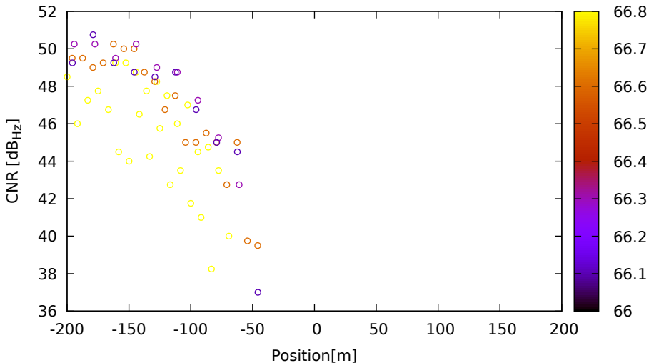
CNR vs position for E09 (E5b) on LeicaGS15 - DOY 262 jam. 1
