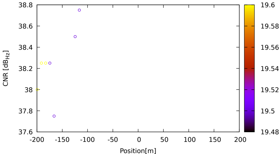
CNR vs position for E11 (E5) on LeicaGS15 - DOY 262 jam. 2
