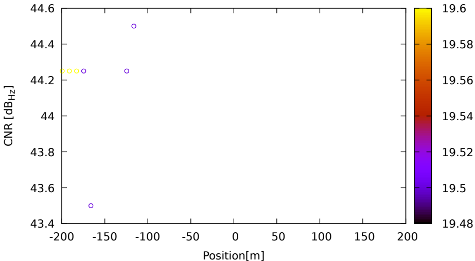
CNR vs position for E11 (E5b) on LeicaGS15 - DOY 262 jam. 2
