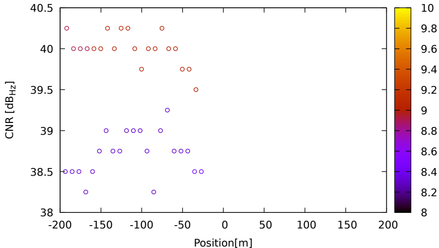
CNR vs position for E15 (E5) on LeicaGS15 - DOY 262 jam. 3
