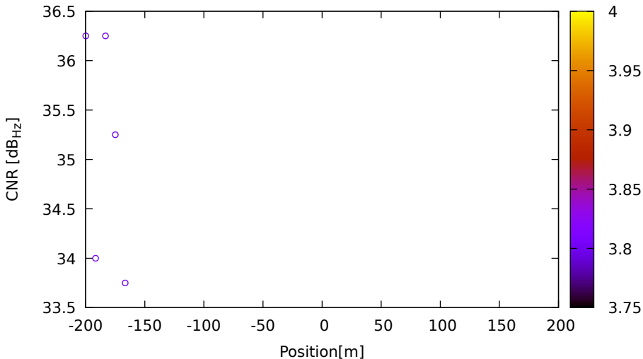
CNR vs position for E30 (E5a) on LeicaGS15 - DOY 262 jam. 1
