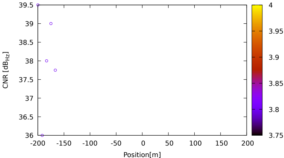
CNR vs position for E30 (E5b) on LeicaGS15 - DOY 262 jam. 1
