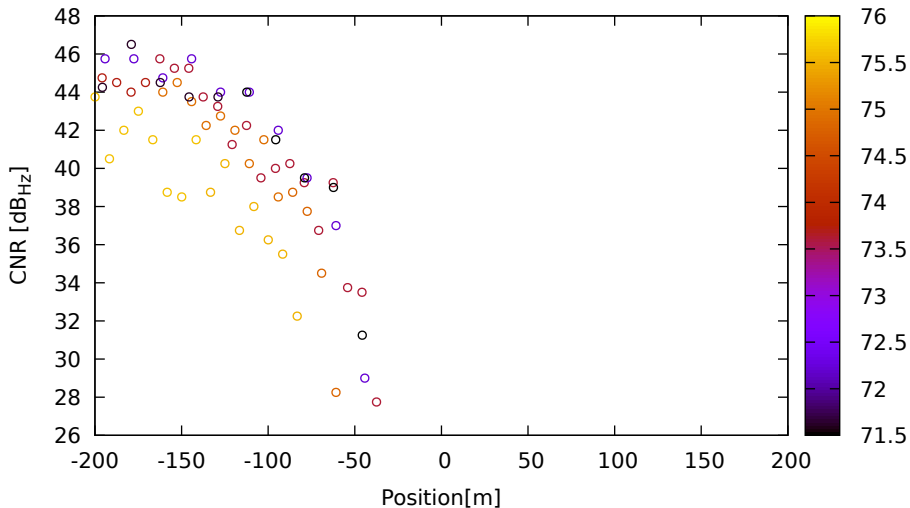
CNR vs position for E36 (E5) on LeicaGS15 - DOY 262 jam. 1
