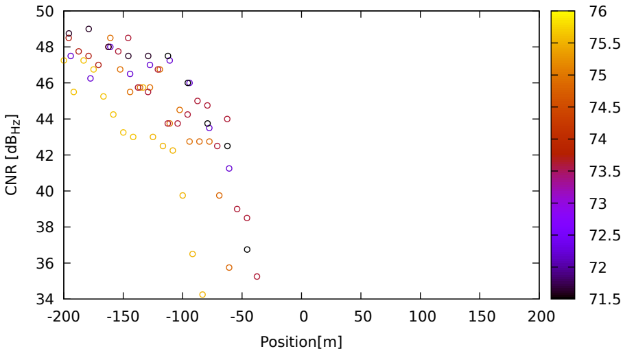
CNR vs position for E36 (E5a) on LeicaGS15 - DOY 262 jam. 1
