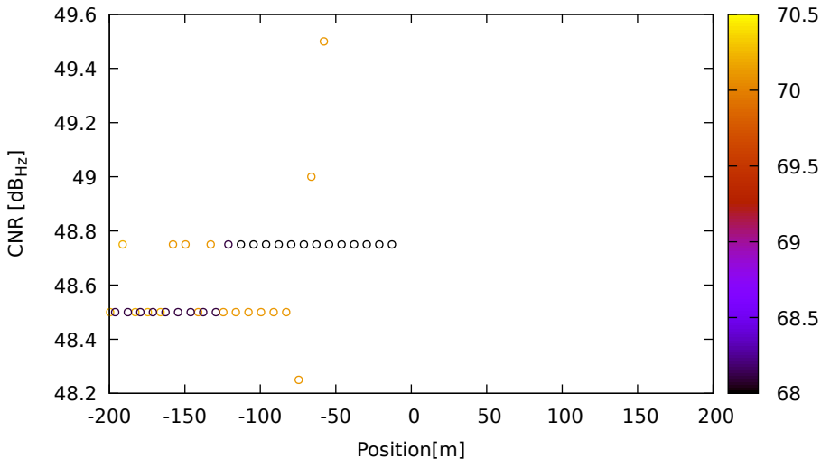
CNR vs position for E36 (E5a) on LeicaGS15 - DOY 262 jam. 2
