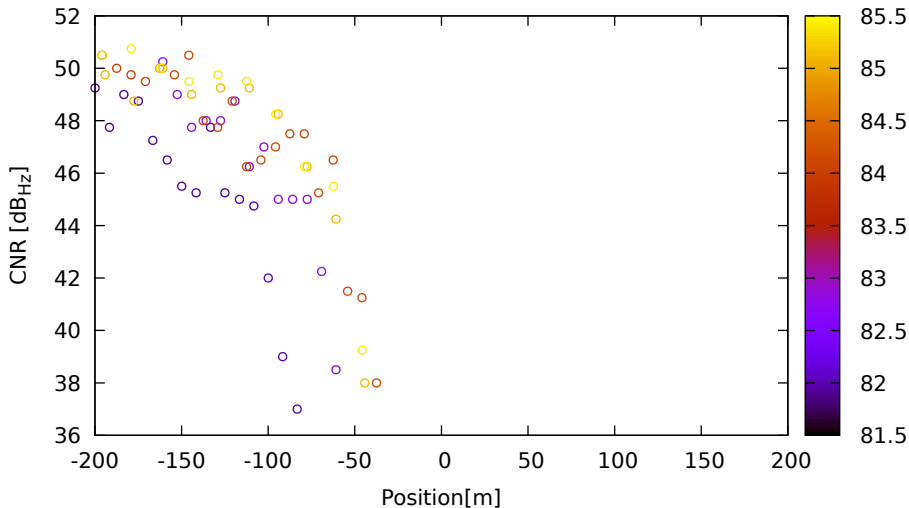
CNR vs position for G01 (L5) on LeicaGS15 - DOY 262 jam. 1
